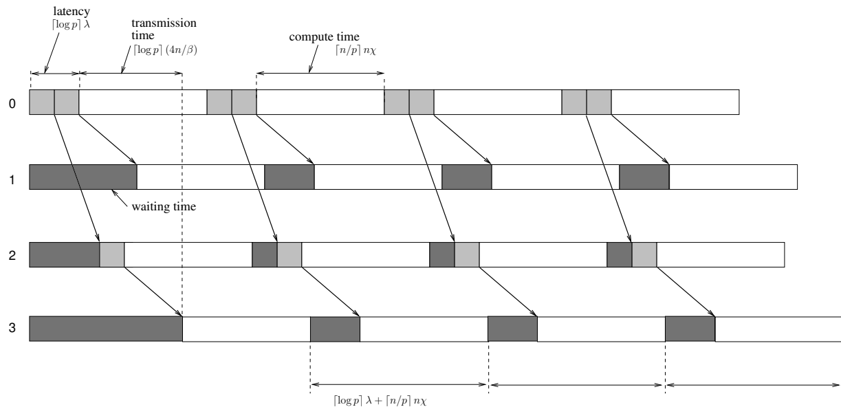
Figure 5.5: Overlap of computation and communication in the first four iterations of the parallel version of Floyd's algorithm, with process 0 responsible for the first 4 rows of the matrix. The figure shows how the transfer of a message overlaps the computation of the sending process.
