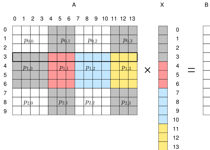
Figure 7.6: Example of the matrix-vector product when the matrix is decomposed into 2D blocks. Rows 3 through 6 of the matrix are color-coded with the parts of the vector that are needed by each subblock. Each row is divided among four processes, each having a unique color. The elements of the vector needed by those processes have the processes' corresponding colors.
