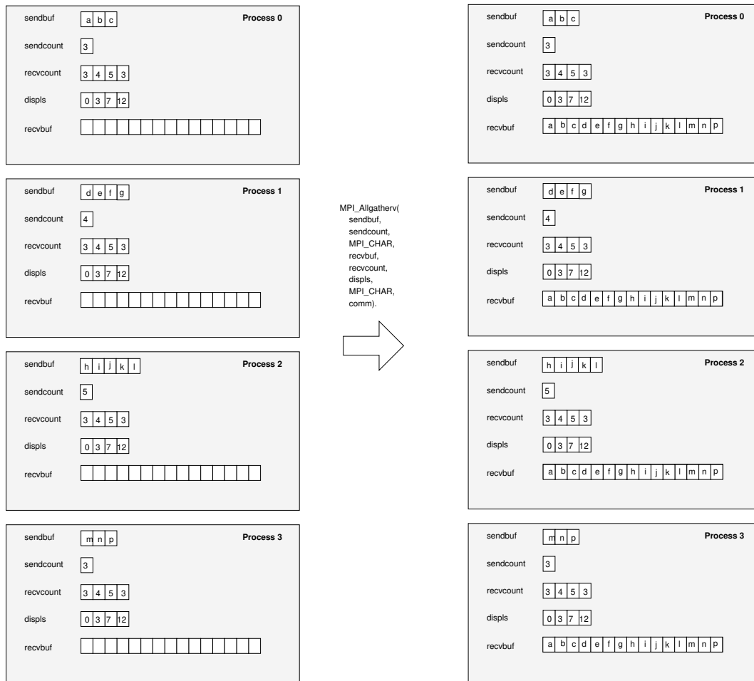
Figure 7.4: Example of four processes using MPI_Allgatherv to gather four different size arrays of data into an identical, replicated array in each process. Each process calls the function with the same values in the arrays passed as recvcount and displs , and when the call returns, all processes have the data in the order specified by those two arrays.
