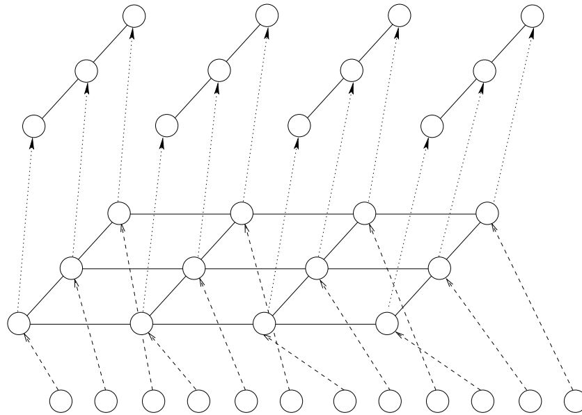
Figure 7.8: The result of splitting a cartesian communicator by columns. After the split, four more communicators exist, and each process is now a part of three different communicator groups, with a rank within each.
