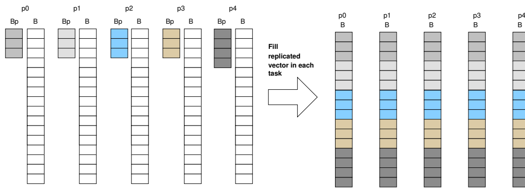
Figure 7.3: Using a block-distributed vector to create a replicated vector in every task. Before the operation, each task has a different block of the vector that it has computed (in B_p ), as well as uninitialized storage for a result vector ( B ). After the operation, the result vector B has been filled with the blocks contributed by all of the tasks, in rank order. This illustrates what has to take place in the final stage of the row-wise block striped algorithm. (The arrays B_p still exist, but are omitted to reduce space in the figure.)
