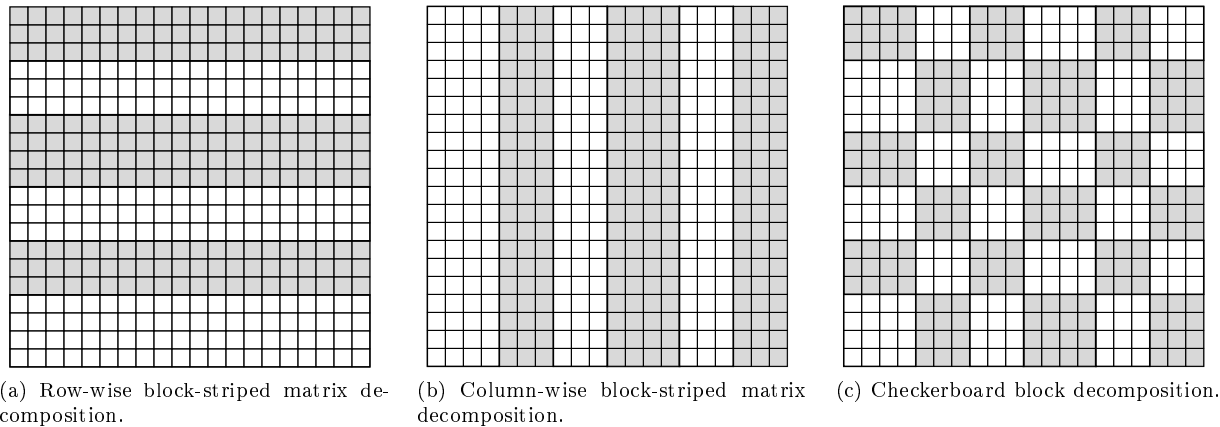
Figure 7.2: Row-wise striped, column-wise striped, and checkerboard block decomposition of a matrix.
