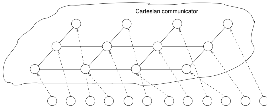
Figure 7.7: Mapping of processes into a 3 \times 4 two-dimensional Cartesian topology by a call to MPI_Cart_create . It is important to remember that after the call the processes exist in the old communicator as well as the new one; they are not removed from the old one. The Cartesian communicator just makes it possible for them to communicate collectively within a grid topology.
